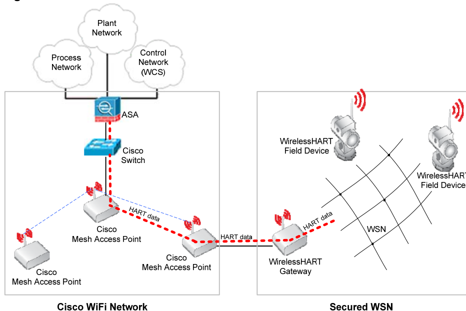
Figure 1 Cisco Secure Wireless Plant Solution
